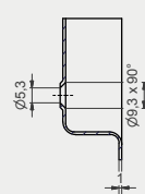
C-C (1:1)
